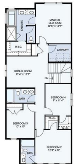
UPPER LEVEL
